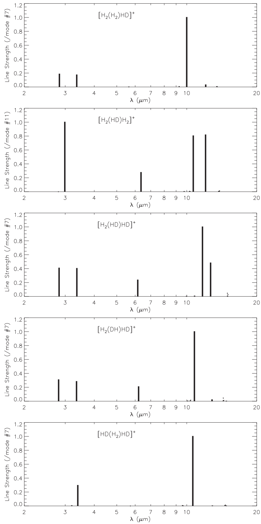
Figure A1. Stick diagram of the mid-IR lines of five isotopomers of \text{H}_6^+ . The line strengths are normalized to that of mode 7 or 11 for each molecule. The E -type modes of the D_{2d} structure are not good approximations to the actual eigenmodes of the molecules (see Section 3.2.1) and they are therefore plotted with dotted lines.
