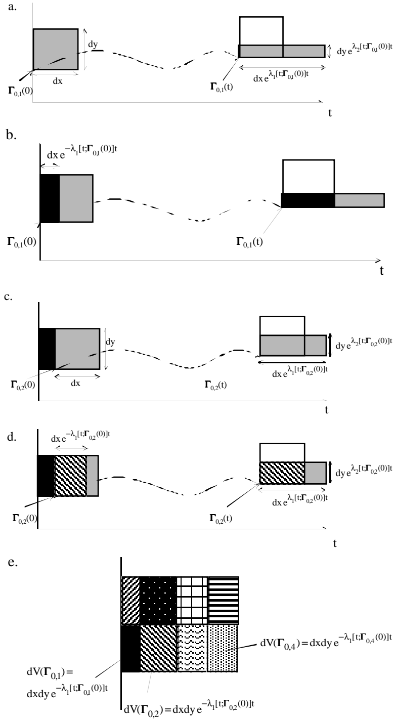
Figure 2 A schematic diagram showing the construction of the partition, or mesh, used to determine phase space averages using Lyapunov weights. For convenience, we assume a two dimensional ostensible phase space, and that there is one positive and one negative time-dependent local Lyapunov exponent for each region in the section of phase space shown. The size of phase volume elements is assumed to be sufficiently small that any curvature in the direction of the eigenvectors can be ignored.
