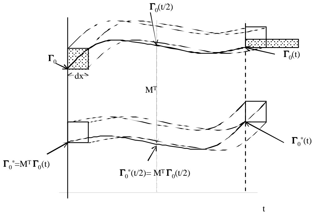
Figure 1 A schematic diagram showing how a trajectory and its conjugate evolve. The square region emanating from \Gamma_0(0) has axes aligned with the eigenvectors of the tangent vector propagator matrix \mathbf{L}[t; \Gamma_0(0)]^T \bullet \mathbf{L}[t; \Gamma_0(0)] . The shaded region thus shows where initial points in this region will propagate to at time t . For illustrative purposes we assume a two dimensional ostensible phase space and that there is one positive time-dependent local Lyapunov exponent (in the x -direction for the
